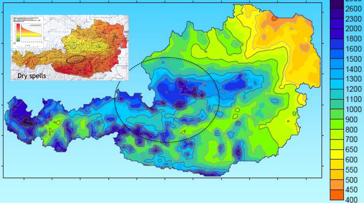
Mean annual precipitation 1961 - 1990 [mm]
