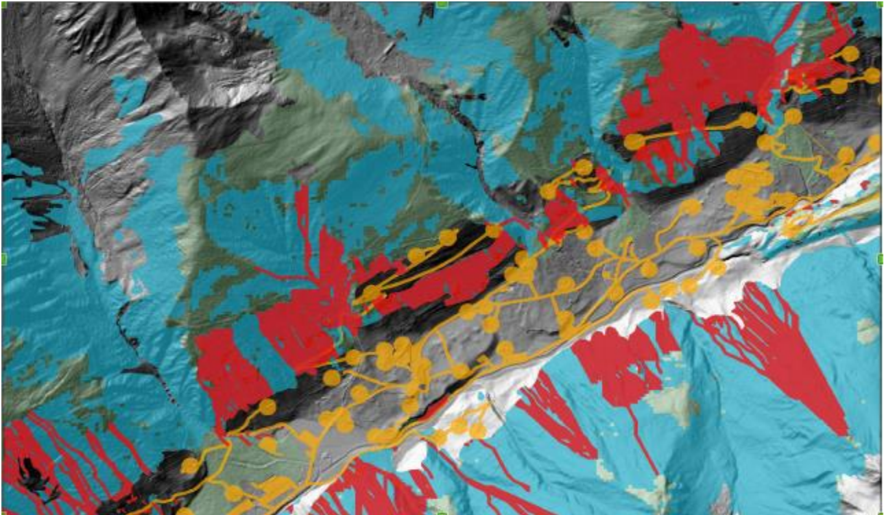
Fig. 13: Rockfall protection: colors as in Fig. 12.
